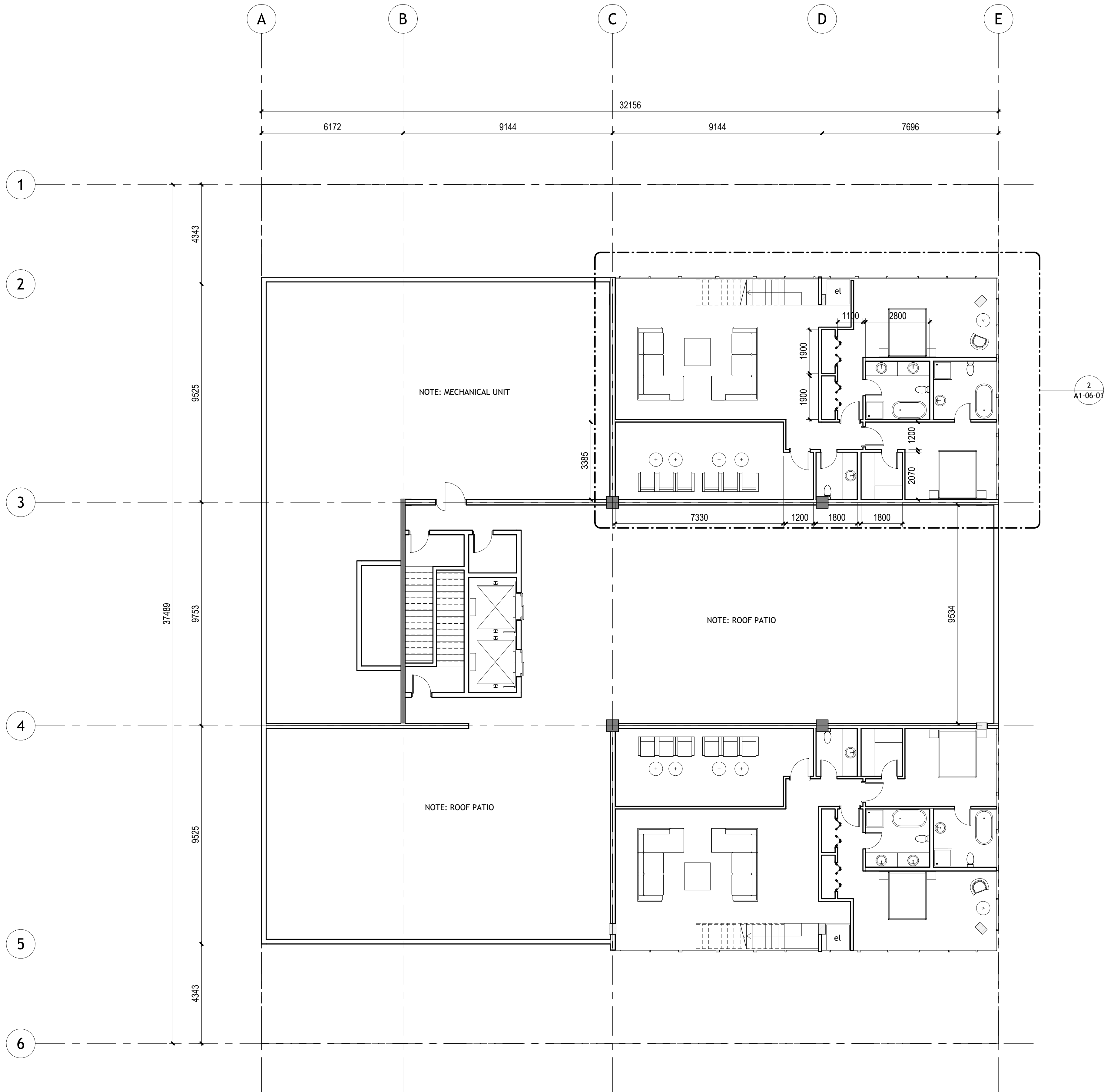
SIXTH FLOOR/ROOF TOP (ARCHITECTURAL PLAN) 1:100
